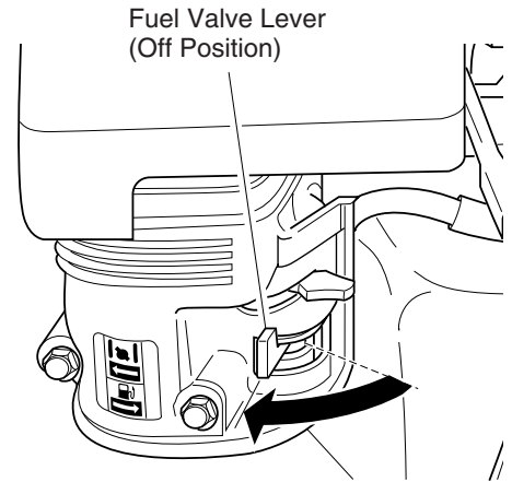
Figure 30 - Fuel Valve Lever Off (Model MGH6500IE Shown)
